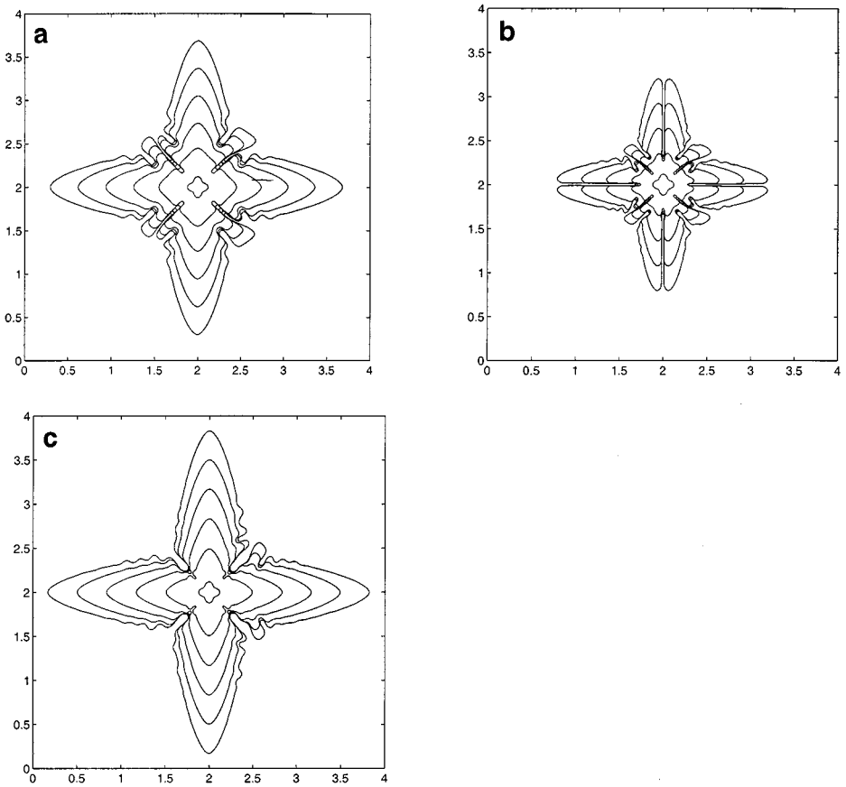
FIG. 25. Fourfold symmetric anisotropy in surface tension. St=0.8 . (a) Higher surface tension case. Surface tension parameter \sigma=0.002 , kinetic parameter \mu=0.0 , surface tension anisotropy A_s=0.4 , and kinetic anisotropy A_k=0.0 . m=4 . t from 0 to 0.05. 500 \times 500 grid. (b) Lower surface tension case. Surface tension parameter \sigma=0.001 , kinetic parameter \mu=0.0 , surface tension anisotropy A_s=0.4 , and kinetic anisotropy A_k=0.0 . m=4 . t from 0 to 0.03. Simulations on an 800 \times 800 grid. (c) Lower surface tension case with kinetic anisotropy. Surface tension parameter \sigma=0.001 , kinetic parameter \mu=0.001 , surface tension anisotropy A_s=0.0 , and kinetic anisotropy A_k=0.4 . m=4 . t from 0 to 0.05. 500 \times 500 grid.
