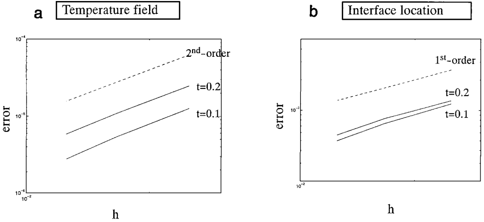
FIG. 15. Errors in the solutions obtained for the melting of the flat interface. The \log(\text{error}) vs \log(h) curves are shown at two different time instants, after 100 time steps ( t = 0.1 ) and after 200 time steps ( t = 0.2 ). (a) L_2 norm of errors in computed temperature field at the two time instants plotted against grid size. The reference second-order line is also shown. (b) L_2 norm of errors in the computed interface location. The reference first-order line is also shown.
