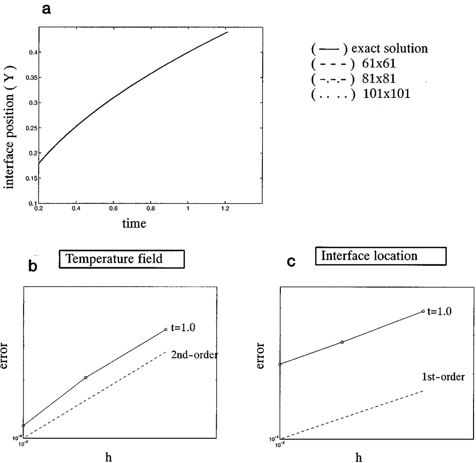
FIG. 18. 2D stable freezing (Stefan) problem. Lower Stefan number, St = 0.1 . (a) Interface position; comparison of exact and computed radius of the freezing circle computed using the grids indicated. (b) log-log plot of the temperature field errors vs grid size. (c) log-log plot of the interface position errors vs grid size.
